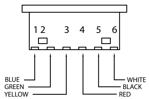
VIEW AA SCALE:5X VIEWED FROM FRONT OF CONNECTOR
