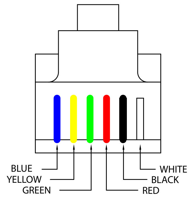
VIEW BB SCALE:6X VIEWED FROM FRONT OF RJ-11
