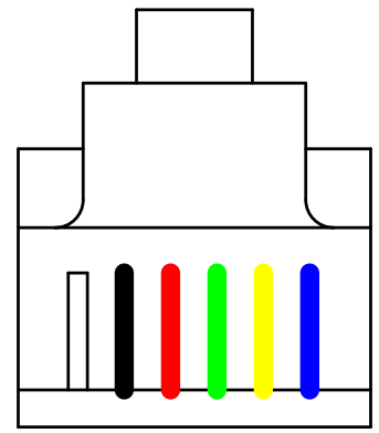
VIEW AA SCALE:6X VIEWED FROM FRONT OF RJ-11
