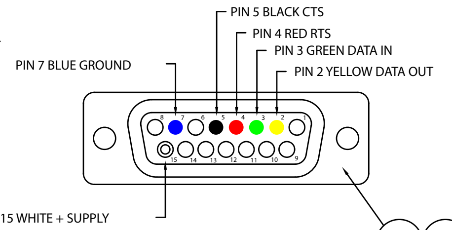
VIEW BB SCALE:2X
